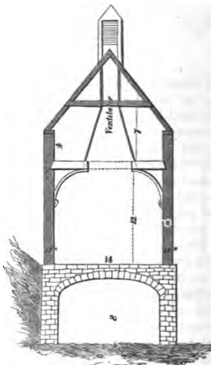
End Section.
